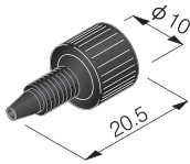
Easy Fitt 10 φ P/N 9001 Carbon reinforced PEEK Quantity: 10
