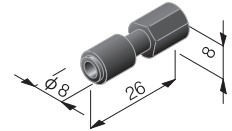
Syringe union P/N 9112 Carbon reinforced PEEK No.10-32UNF, Syringe port Quantity: 1
