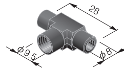
Reducing tee P/N 9107 Carbon reinforced PEEK No.10-32UNF, M8 Quantity: 1
