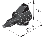
Easy Fitt Type 2 P/N 9130 Carbon reinforced PEEK Quantity: 10
