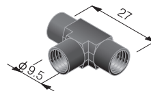
Tee P/N 9121 Carbon reinforced PEEK M8 Quantity: 1
