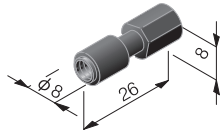
Union P/N 9005 Carbon reinforced PEEK No.10-32UNF Quantity: 1
