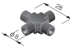
Cross P/N 9007 Carbon reinforced PEEK No.10-32UNF Quantity: 1
