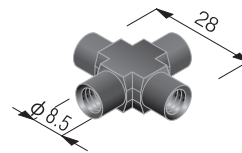
Cross P/N 9109 Carbon reinforced PEEK No.1/4-28UNF Quantity: 1
