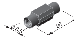
1/4-28 Flat seal union P/N 9101 Carbon reinforced PEEK No.1/4-28UNF Quantity: 1
