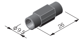
Union P/N 9111 Carbon reinforced PEEK M8 Quantity: 1
