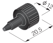
Easy Fitt 12 φ P/N 9002 Carbon reinforced PEEK Quantity: 10
