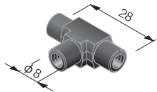
Tee P/N 9006 Carbon reinforced PEEK No.10-32UNF Quantity: 1
