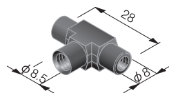
Reducing tee P/N 9108 Carbon reinforced PEEK No.10-32, 1/4-28UNF Quantity: 1
